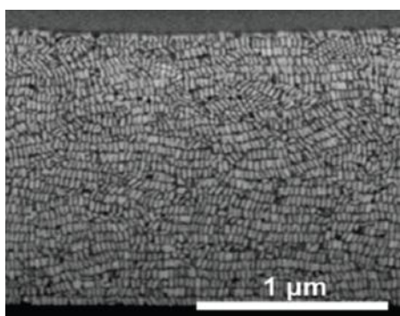
SEM image of the cross-section of a gold nanorod supercrystal
